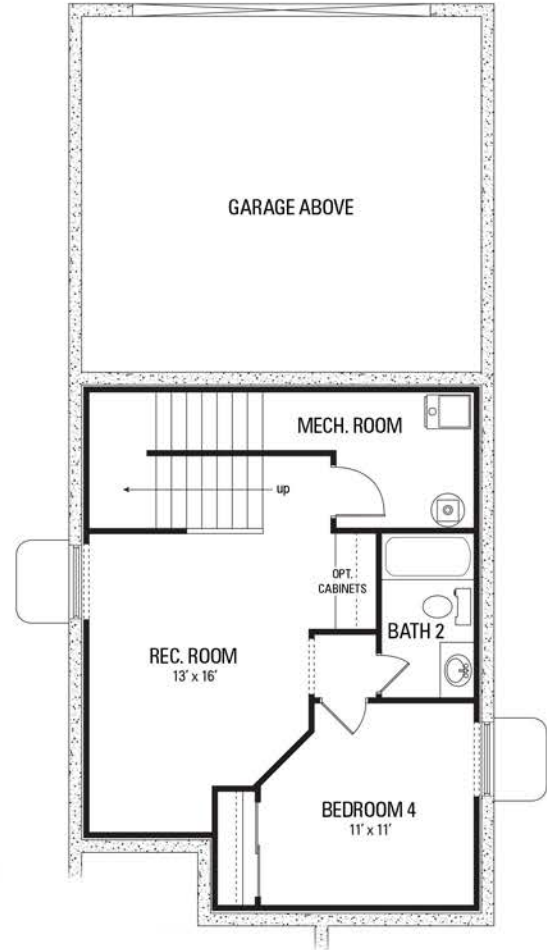
OPT. FINISHED BASEMENT 587 SQ FT
