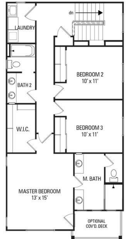
UPPER LEVEL 996 SQ. FT
