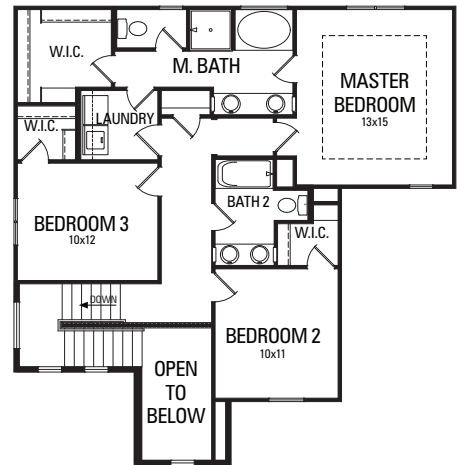
UPPER LEVEL 968 SQ. FT
